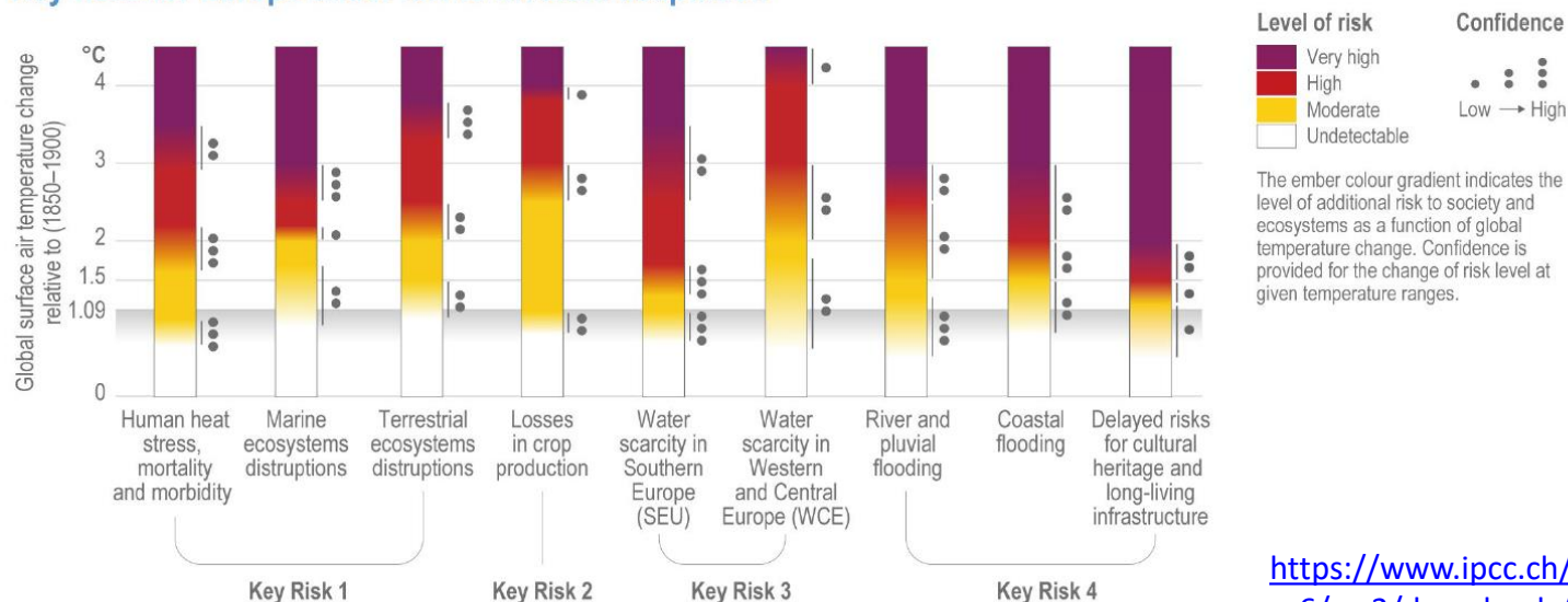
Figure 2: Burning ember diagrams for key risks for Europe with low to medium adaptation. {Figure 13.28}
